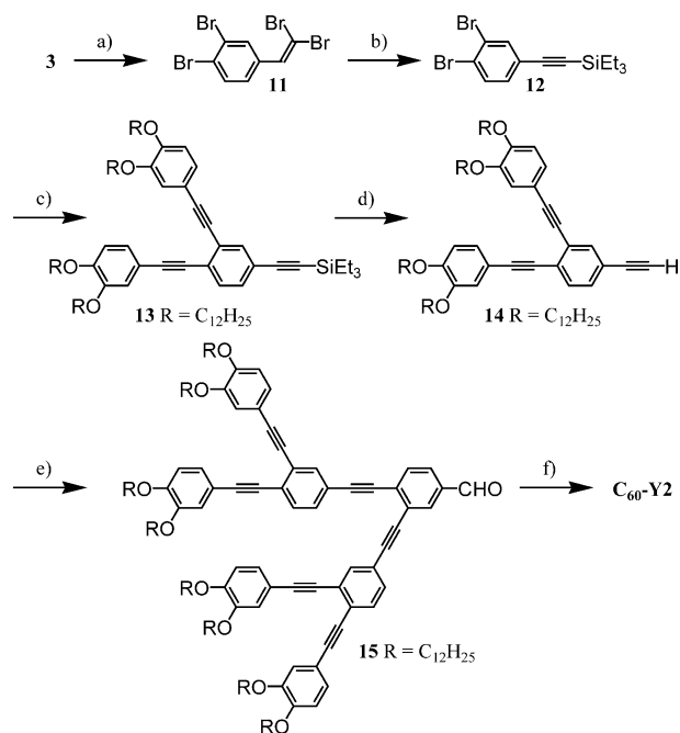
Scheme 3. Reagents and conditions: (a) \text{CBr}_4 , \text{PPh}_3 , \text{Zn} , \text{CH}_2\text{Cl}_2 , 0^\circ\text{C} to room temp. (95%); (b) \text{LDA} , \text{THF} , -78^\circ\text{C} , then \text{TESCl} , \text{THF} , -78^\circ\text{C} (63%); (c) 1 , \text{Pd}(\text{PPh}_3)_2\text{Cl}_2 , \text{CuI} , \text{PPh}_3 , \text{Et}_3\text{N} , \text{THF} , 65^\circ\text{C} (99%); (d) \text{TBAF} , \text{THF} , 0^\circ\text{C} (92%); (e) 3 , \text{Pd}(\text{PPh}_3)_2\text{Cl}_2 , \text{CuI} , \text{PPh}_3 , \text{Et}_3\text{N} , \text{THF} , 65^\circ\text{C} (84%); (f) \text{C}_{60} , N -methylglycine, toluene, \Delta (50%).
