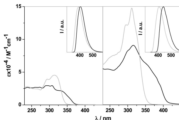
Figure 5. Absorption and normalized fluorescence spectra (inset) of (a) Y1 (black), G1 (grey); (b) Y2 (black), G2 (grey); CH_2Cl_2 , 298 K. Emission spectra were recorded upon excitation at the absorption maximum (O.D. = 0.1).
