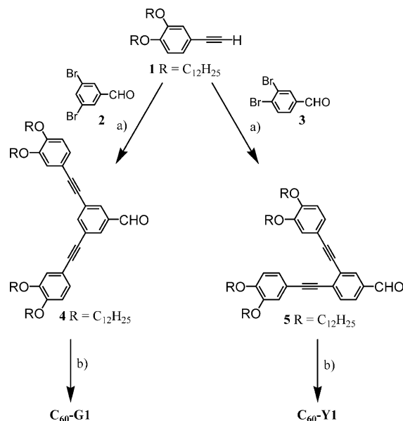
Scheme 1. Reagents and conditions: (a) Pd(PPh 3 ) 2 Cl 2 , CuI, PPh 3 , Et 3 N, THF, 65 °C ( 4 : 86%, 5 : 82%); (b) C 60 , N -methylglycine, toluene, Δ ( C 60 -G1 : 61%, C 60 -Y1 : 46%).
