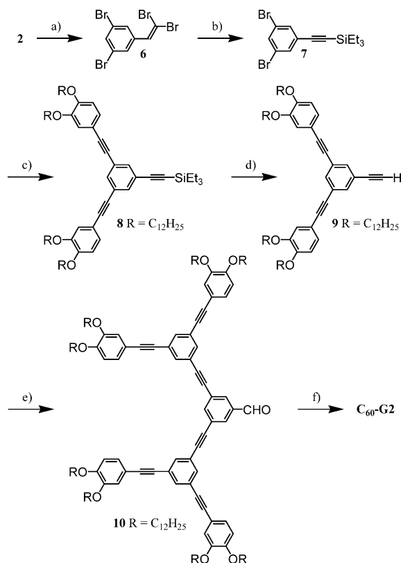
Scheme 2. Reagents and conditions: (a) \text{CBr}_4 , \text{PPh}_3 , \text{Zn} , \text{CH}_2\text{Cl}_2 , 0^\circ\text{C} to room temp. (95%); (b) \text{LDA} , \text{THF} , -78^\circ\text{C} , then \text{TESCl} , \text{THF} , -78^\circ\text{C} (70%); (c) 1 , \text{Pd}(\text{PPh}_3)_2\text{Cl}_2 , \text{CuI} , \text{PPh}_3 , \text{Et}_3\text{N} , \text{THF} , 65^\circ\text{C} (99%); (d) \text{K}_2\text{CO}_3 , \text{THF} , \text{MeOH} , room temp. (91%); (e) 2 , \text{Pd}(\text{PPh}_3)_2\text{Cl}_2 , \text{CuI} , \text{PPh}_3 , \text{Et}_3\text{N} , \text{THF} , 65^\circ\text{C} (96%); (f) \text{C}_{60} , N -methylglycine, toluene, \Delta (52%).
