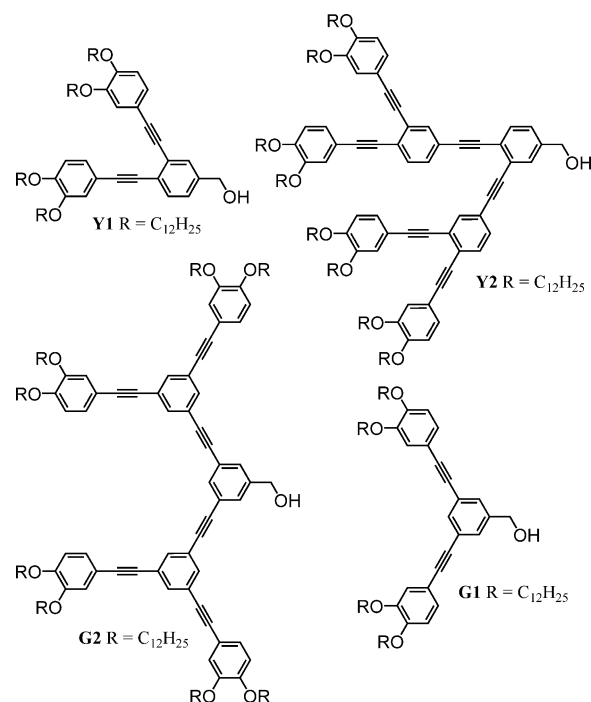
Figure 3. Model compounds G1 , G2 , Y1 , and Y2 .
