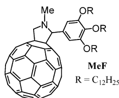
Figure 4. Model compound MeF .
