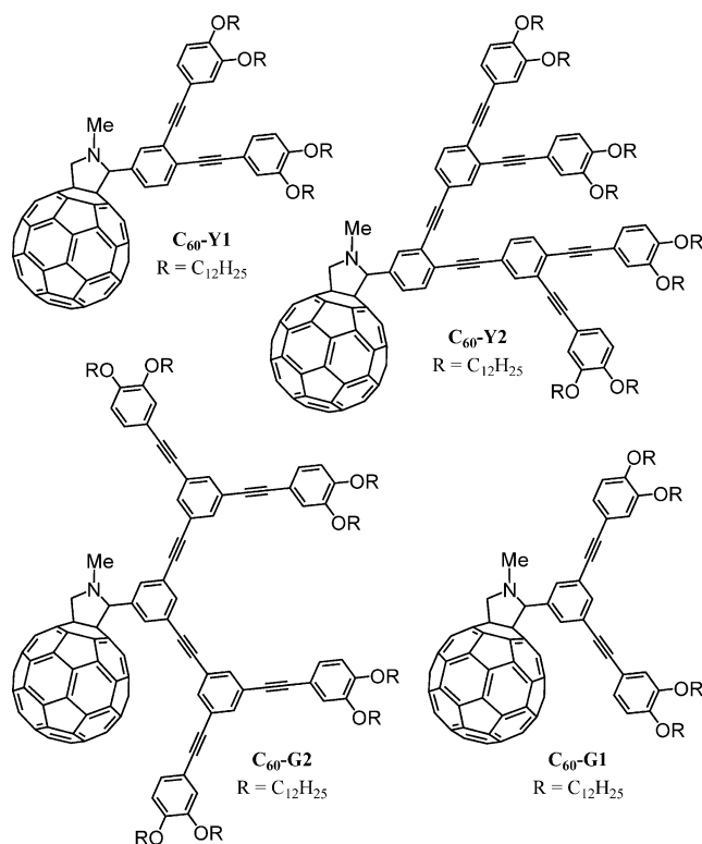
Figure 1. Compounds C 60 -G1 , C 60 -G2 , C 60 -Y1 , and C 60 -Y2 .
