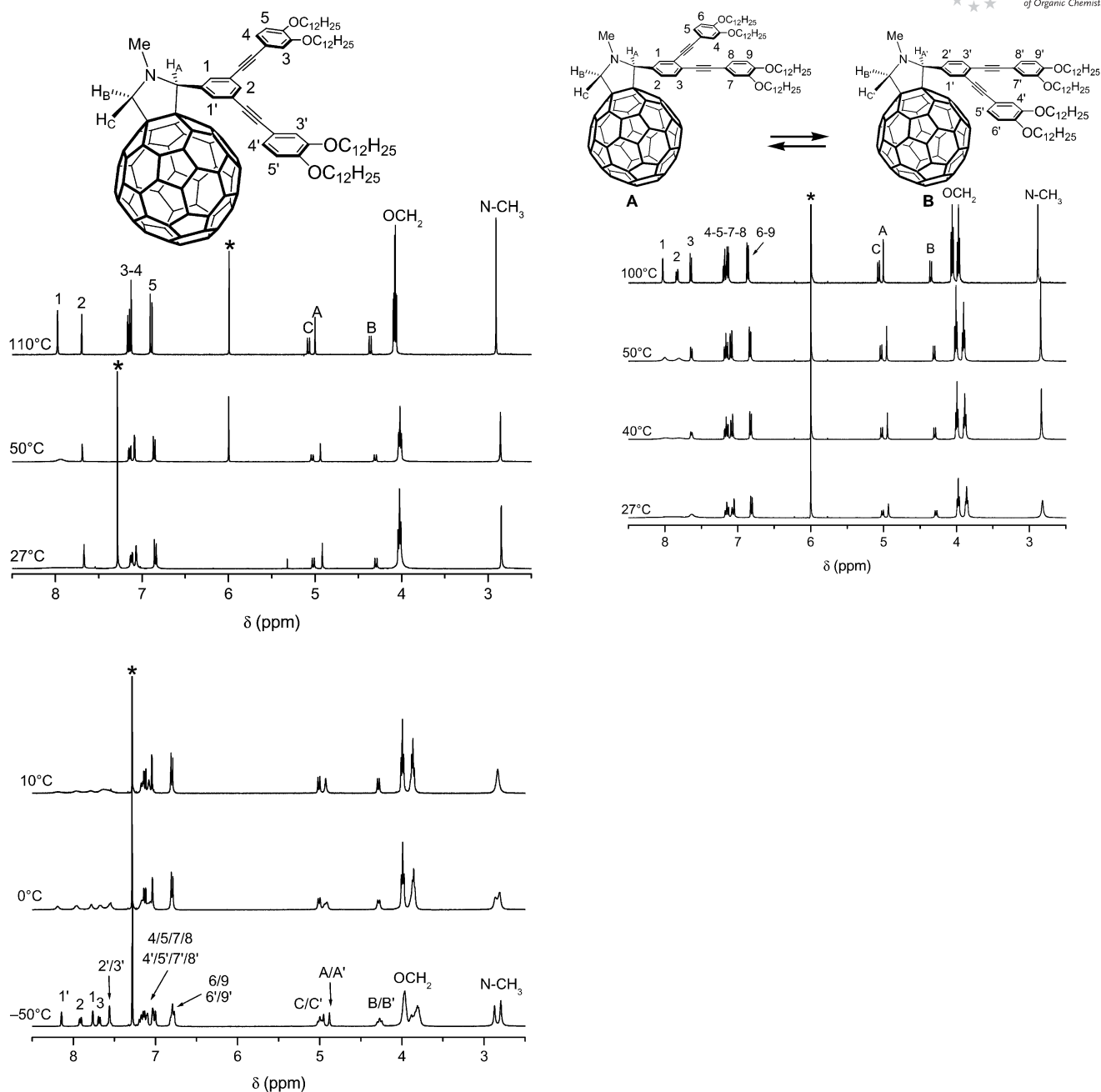
Figure 2. (top left) ^1\text{H} NMR spectra (400 MHz) of C 60 - G1 recorded in \text{C}_2\text{D}_2\text{Cl}_4 at 110 and 50 °C, and in \text{CDCl}_3 at room temperature (* solvent peak); (top right) ^1\text{H} NMR spectra (400 MHz) of C 60 - Y1 recorded in \text{C}_2\text{D}_2\text{Cl}_4 at 100, 50, 40 and 27 °C (* solvent peak); (bottom) ^1\text{H} NMR spectra (400 MHz) of C 60 - Y1 recorded in \text{CDCl}_3 at 10, 0, and -50 °C (* solvent peak; for the numbering, see Figure 2 top right).
