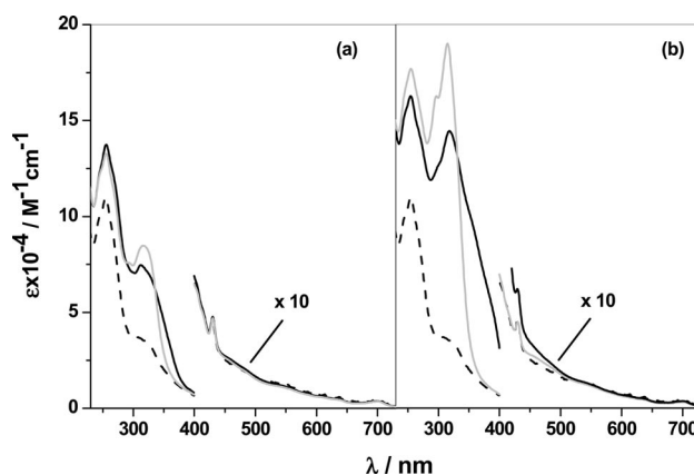
Figure 6. Absorption spectra of dyad compounds: (a) fulleropyrrolidine reference MeF (dashed), C 60 Y1 (black), C 60 G1 (grey); (b) fulleropyrrolidine reference MeF (dashed), C 60 Y2 (black), C 60 G2 (grey); CH_2Cl_2 , 298 K. Beyond 400 nm, spectra are increased by a factor of 10 for display purposes.
